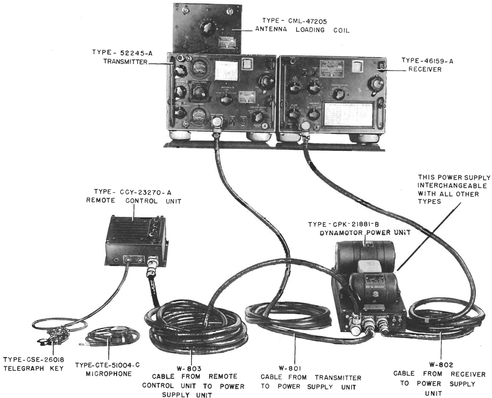
Figure 1-1 Complete TCS Equipment
